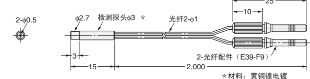
E32-D22R
