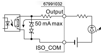
驱动 LED 灯
